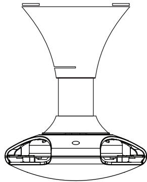
Motor Assembly with Downrod, Coupling Cover, Rod Cover and Canopy
